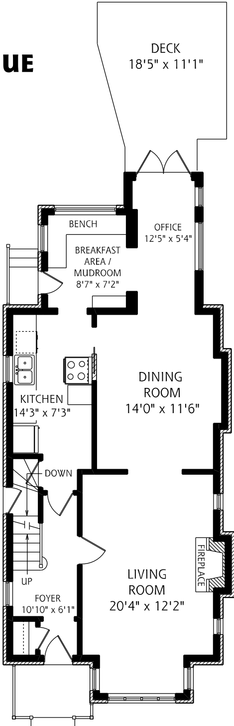
MAIN FLOOR 885 SQUARE FEET
