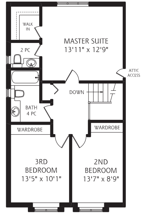
SECOND FLOOR 735 SQUARE FEET
